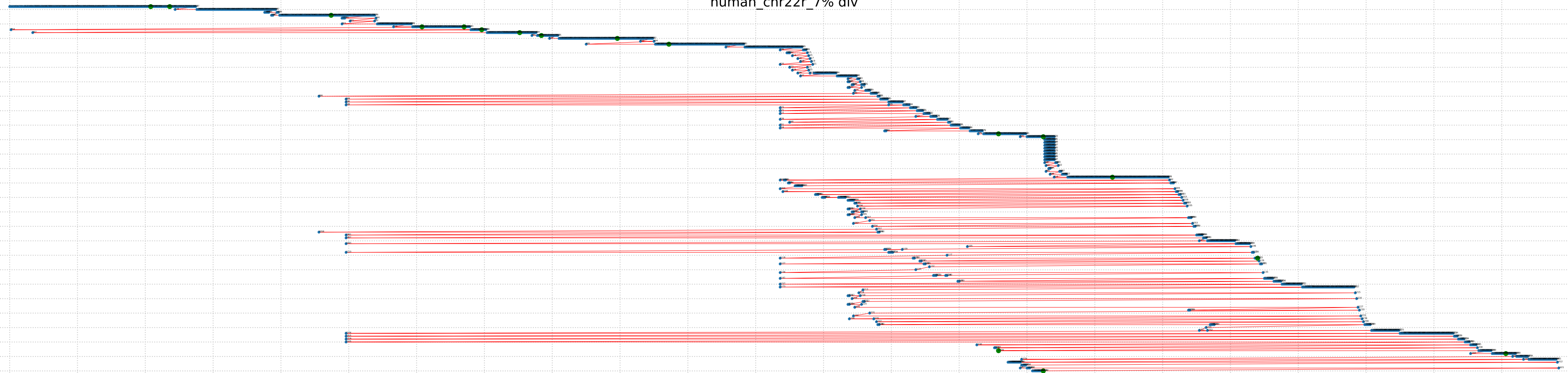
human_chr22r_7% div
