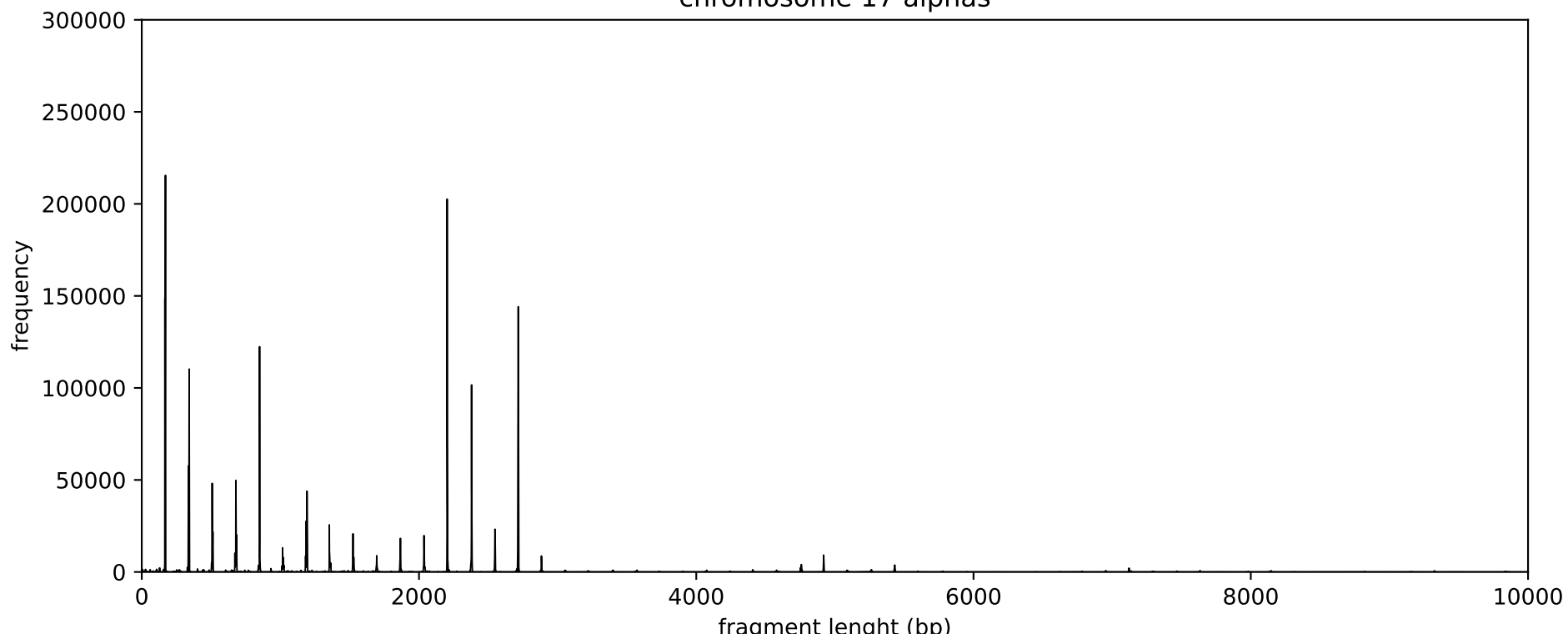
chromosome 17 alphas
