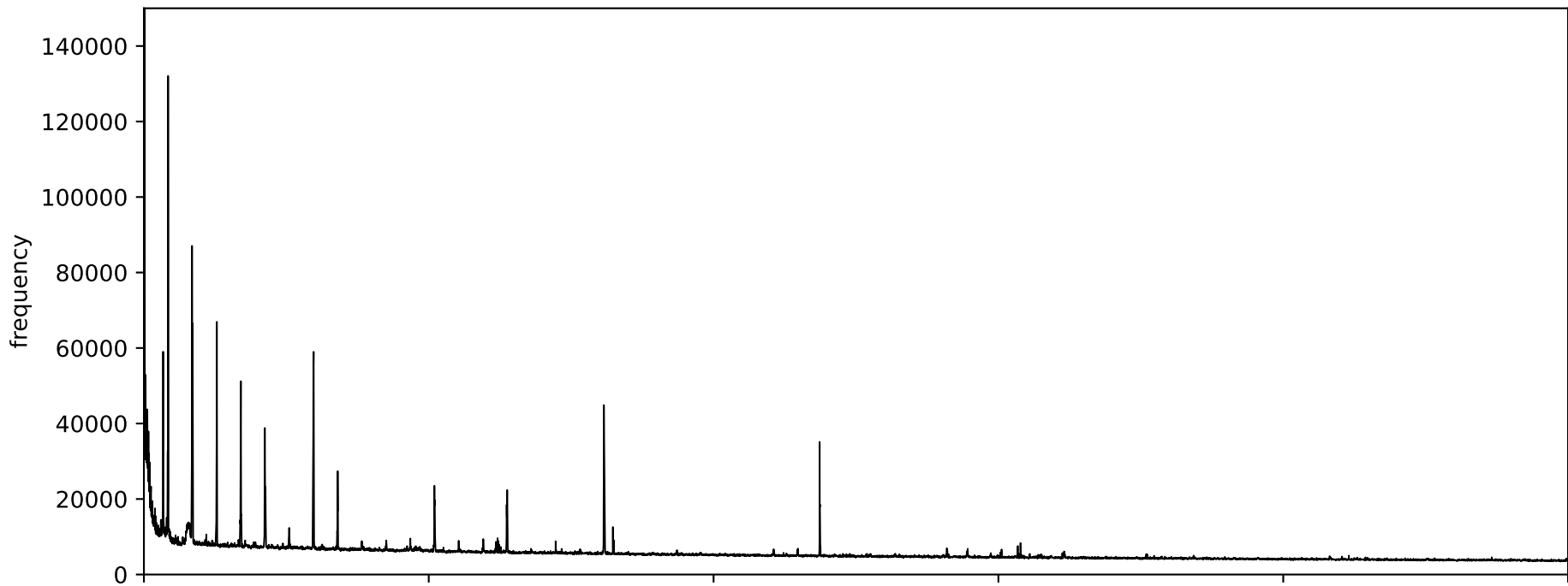
chromosome 04 alphas
