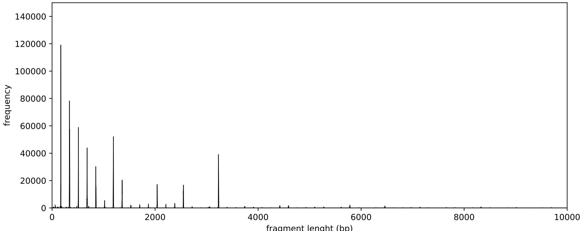
chromosome 04 alphas
