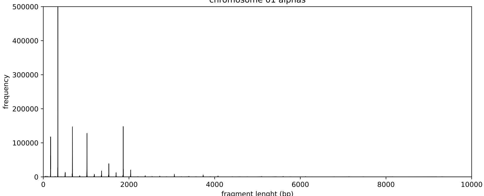
chromosome 01 alphas
