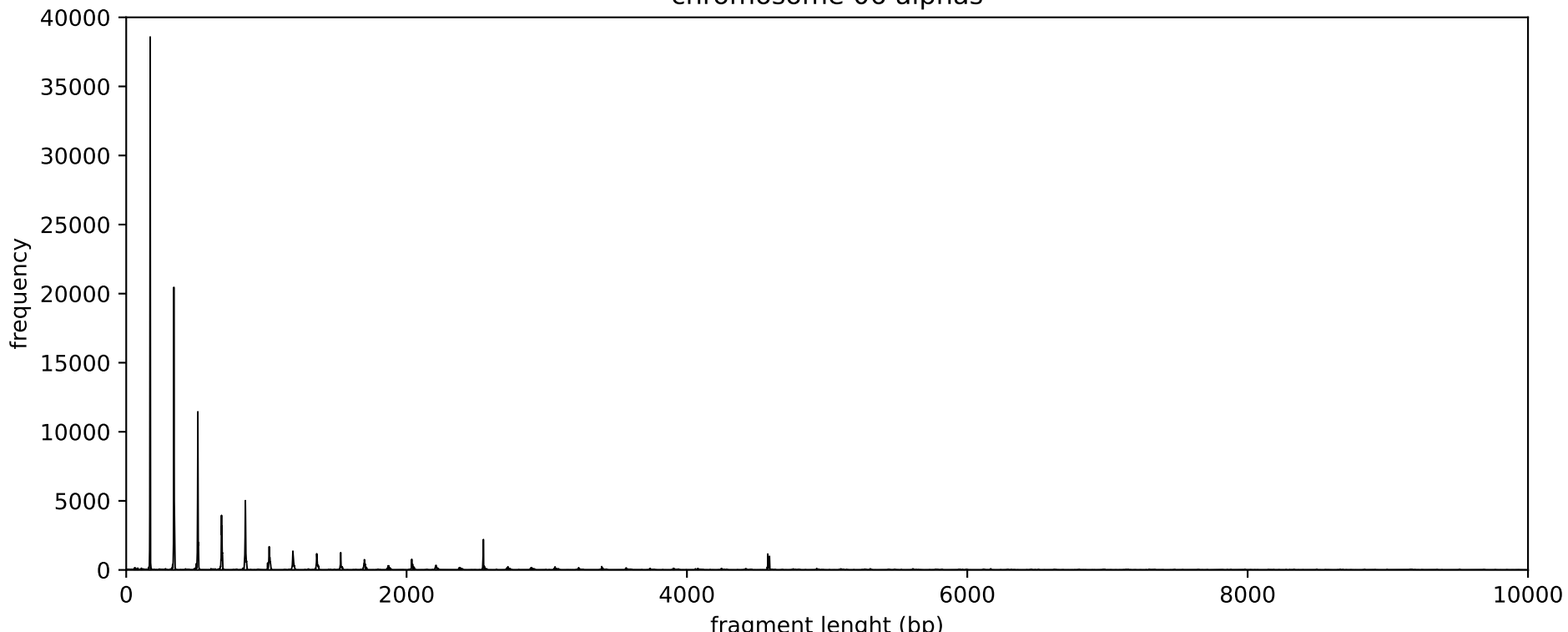
chromosome 06 alphas
