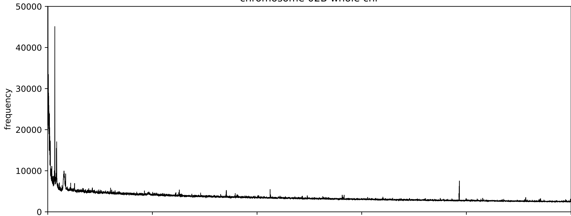
chromosome 02B alphas
