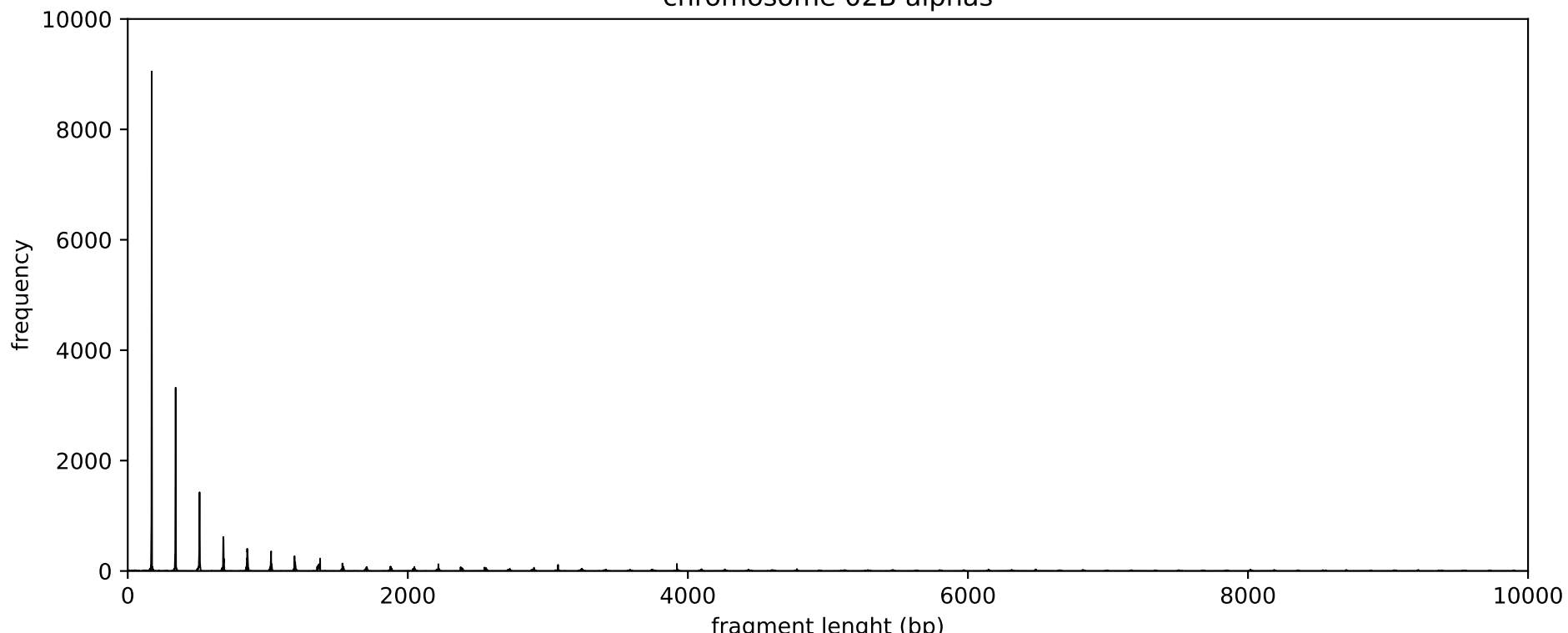
chromosome 02B alphas
