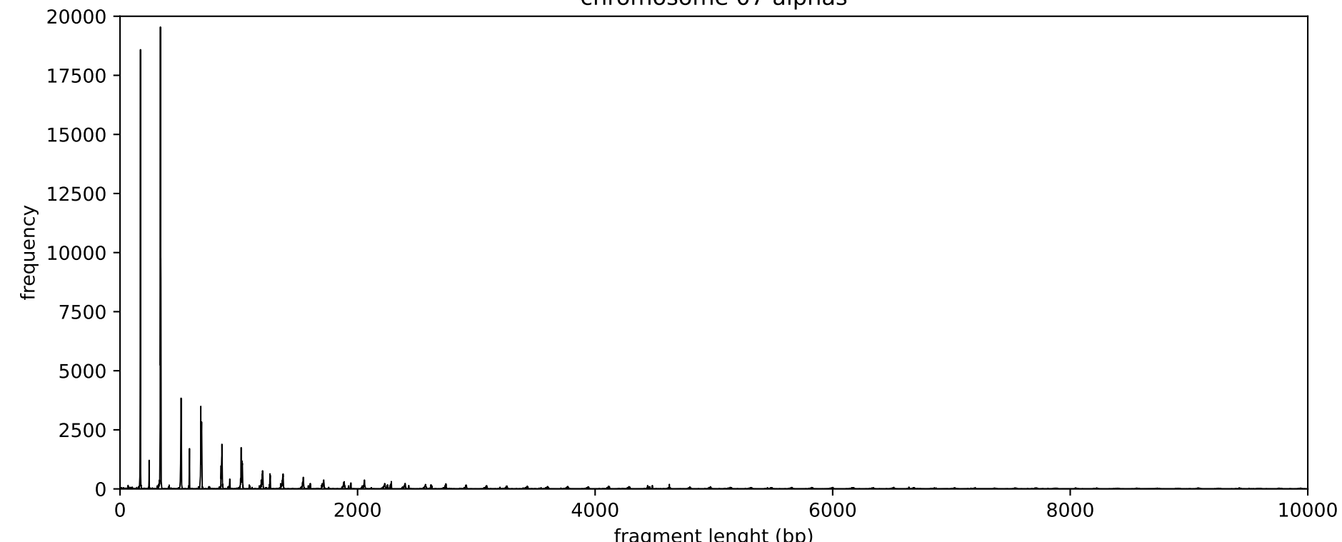
chromosome 07 alphas
