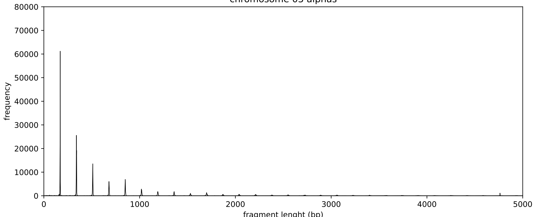
chromosome 03 alphas
