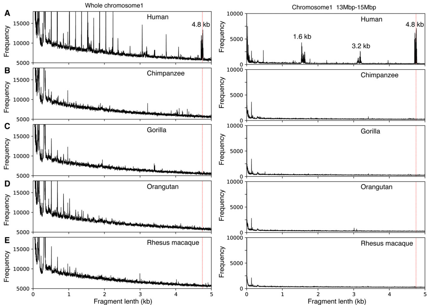
Figure 2. Global repeat map diagrams for National Center for Biotechnology Information (2022) primate genome assemblies.
