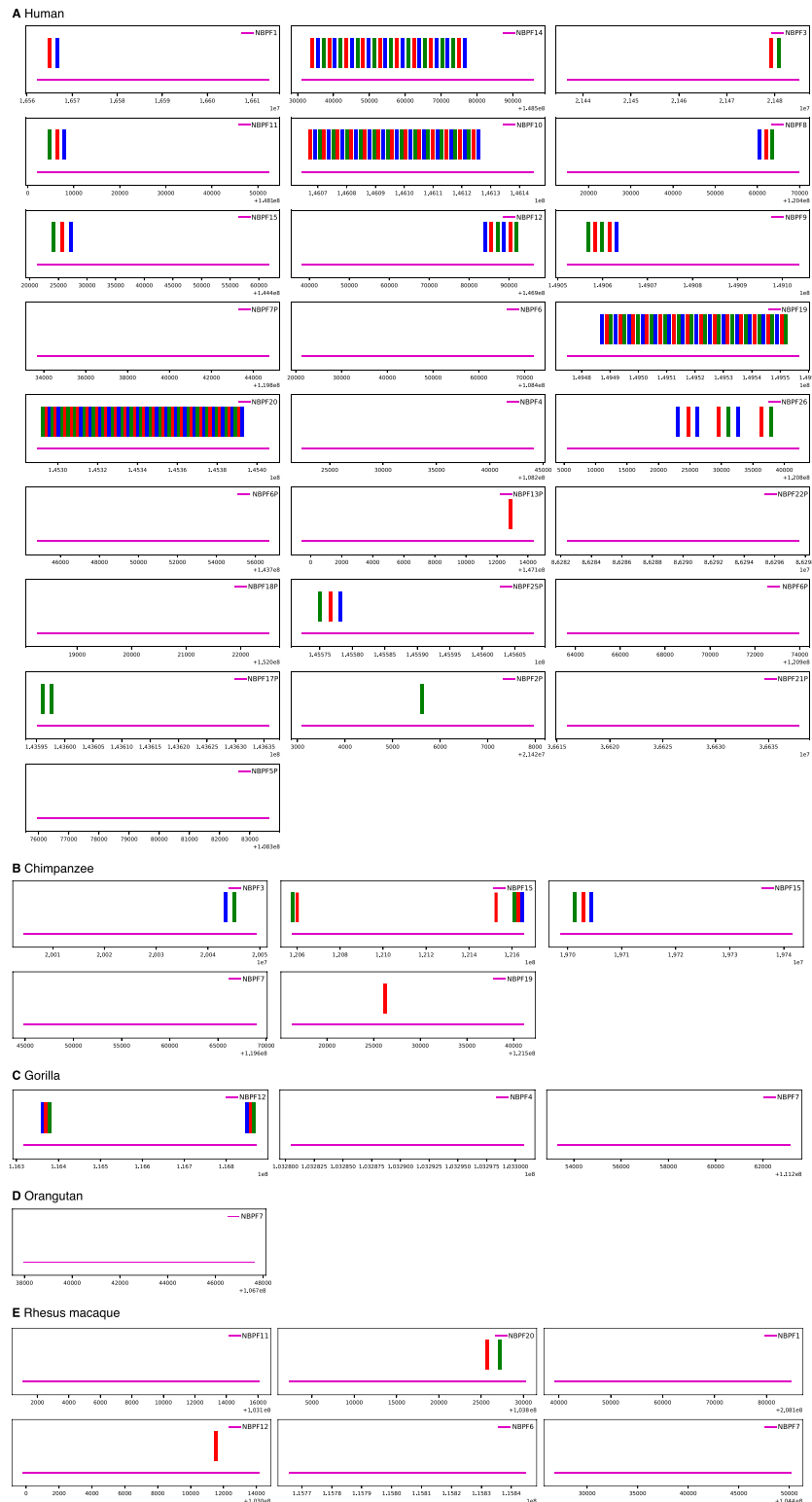
Figure 3. NBPF monomer distribution along the National Center for Biotechnology Information (2022) genome assemblies.
